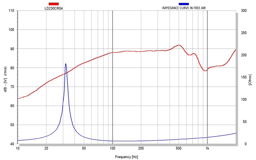
ATOHM LD230CR04 Signal 2.83Vrms@1m
