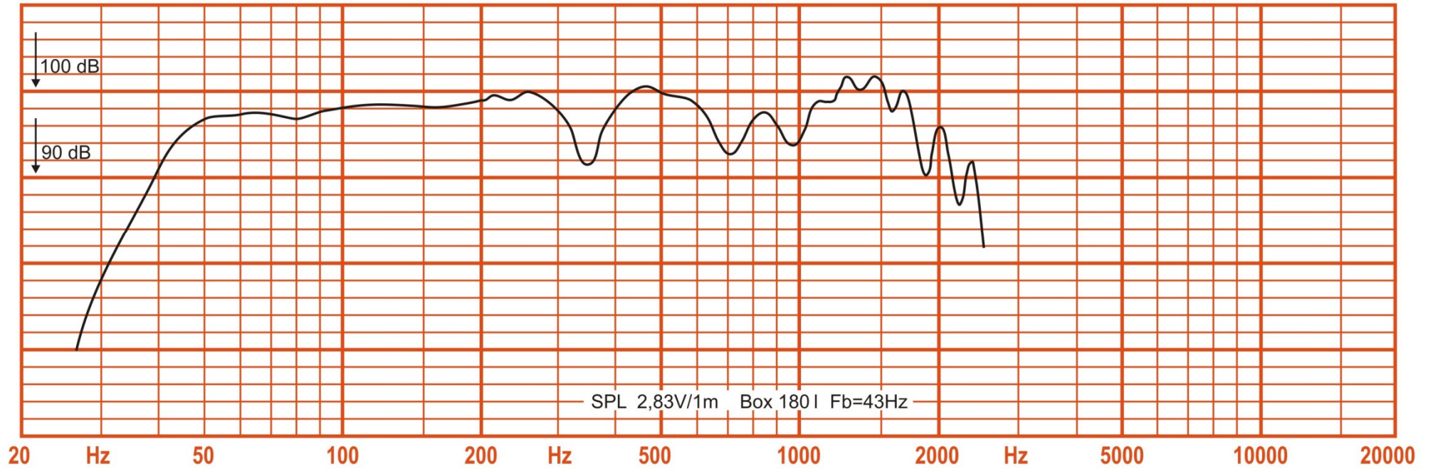
Frequency Responce
