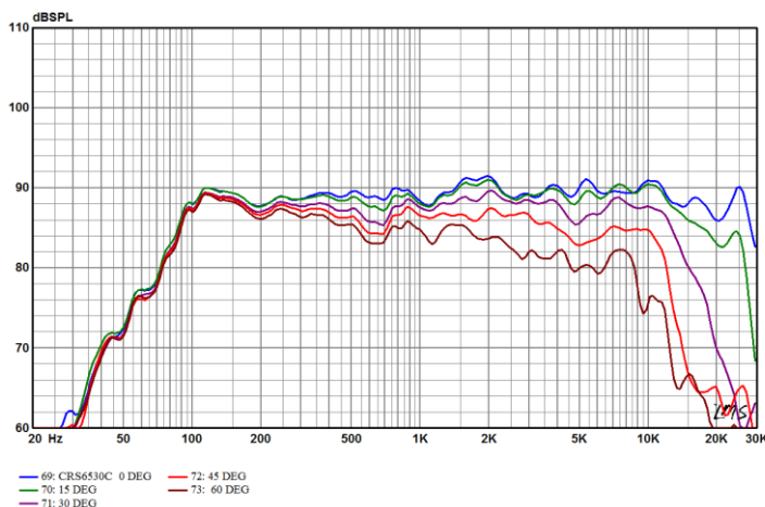
Directivity response curves of CRS6530C with recommended XO in V_b=6.5 L/ F_b=65 Hz vented box, free field.
