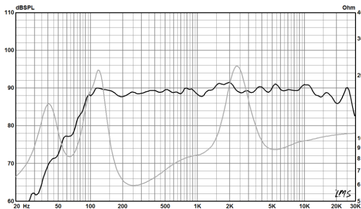
Combined frequency response and impedance of 6CRS5130-R with recommended XO in V_b=6.5 L/ F_b=65 Hz vented box, free field.
