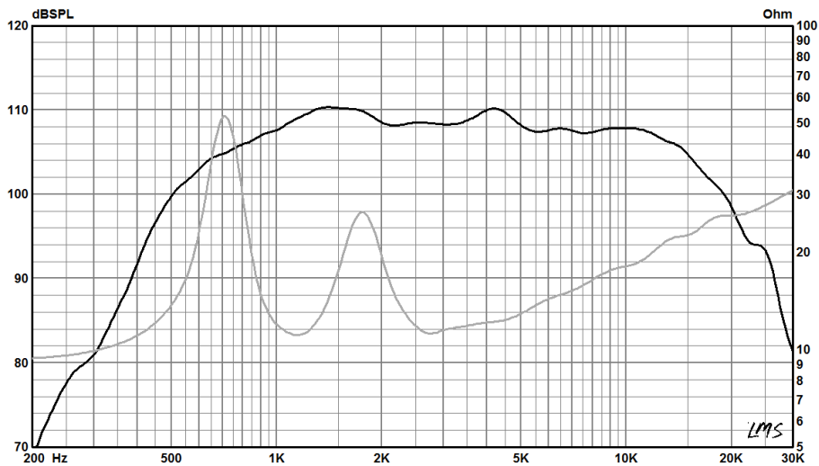
Frequency response and impedance of 951 NeoPB-16 on specified horn, free field 3 .
