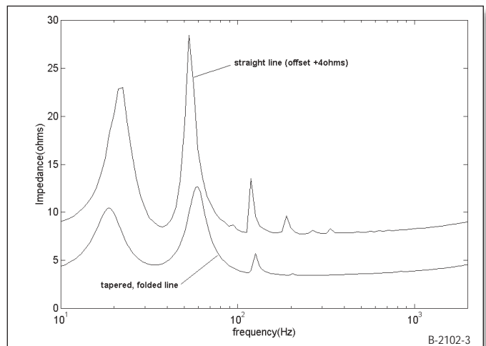
FIGURE 3: Unfilled transmission-line impedance comparison.
