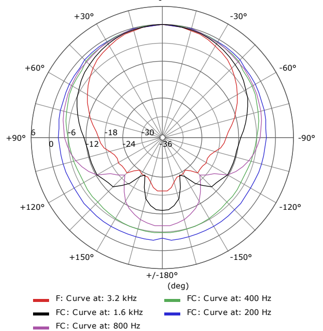
Z001920-W polar diagram
