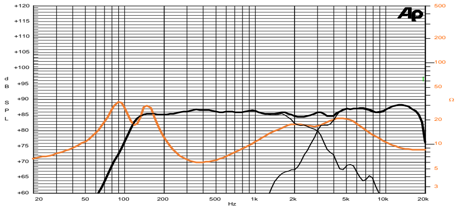
Frequency Response on 2 Lt @ 120 Hz Vented Box @ 1W, 1m Free Air Impedance
